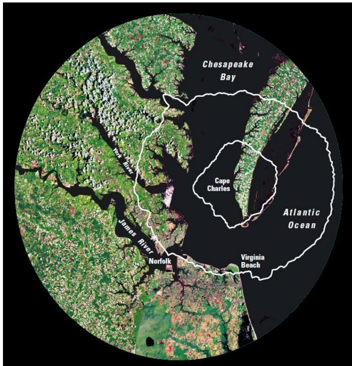
Figure 7: A Bolide Bulls-Eye. Source: USGS
