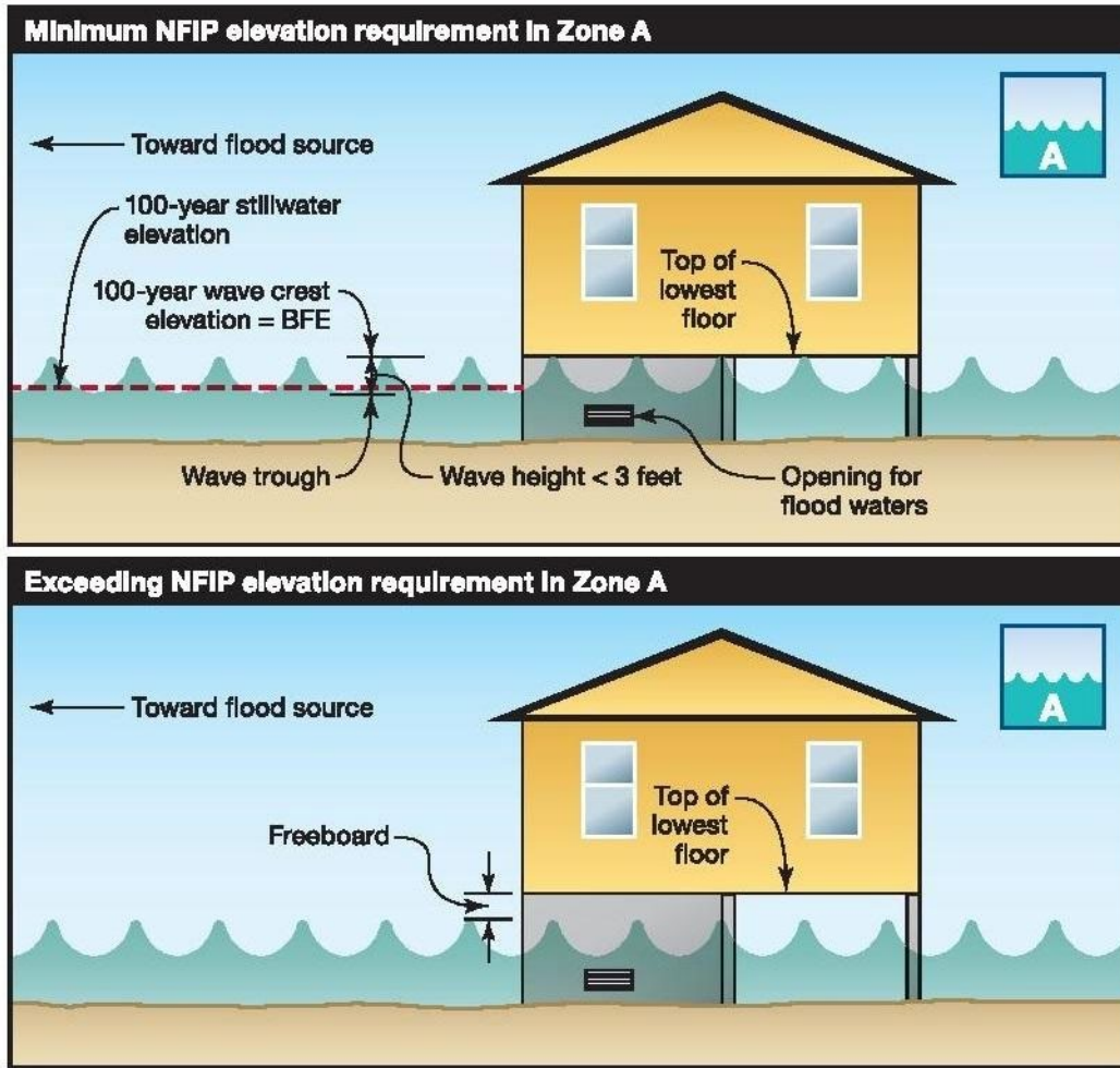
Figure 11: Recommended Elevation for Buildings in Zone A Compared to Minimum Requirements Source: FEMA Coastal Construction Manual, 2011
