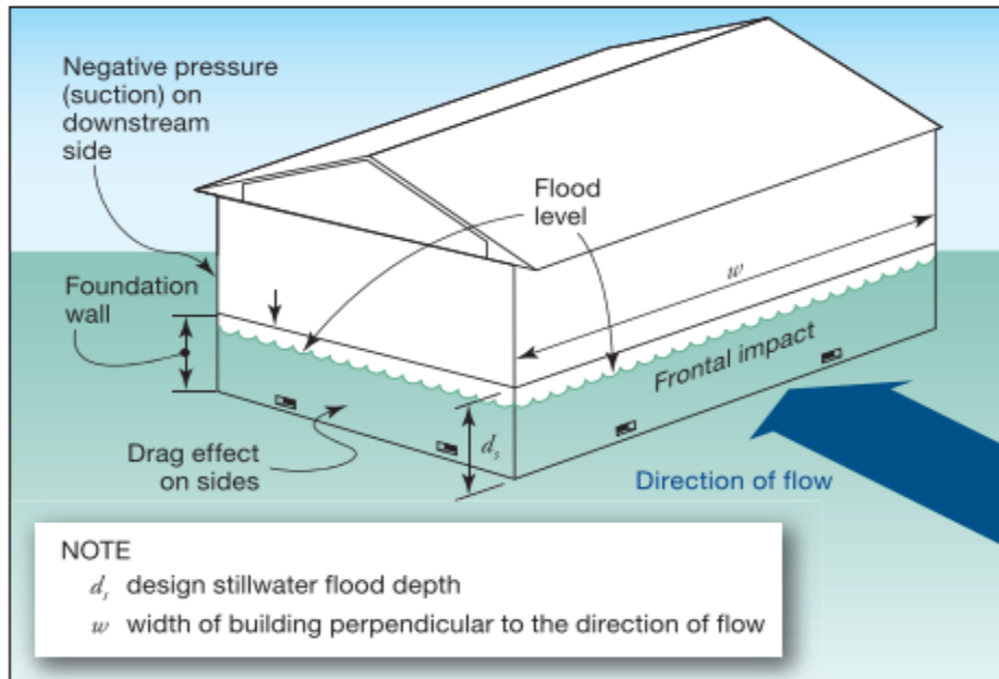
Figure 7: Hydrodynamic building loads
